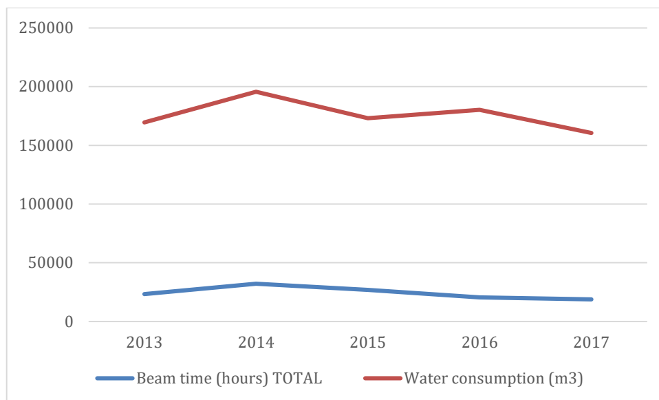
Figure 20: Water consumption in m 3 and beam time in hours (data from ALTO, ECT*, GANIL, GSI, LNL and NLC Warsaw)
