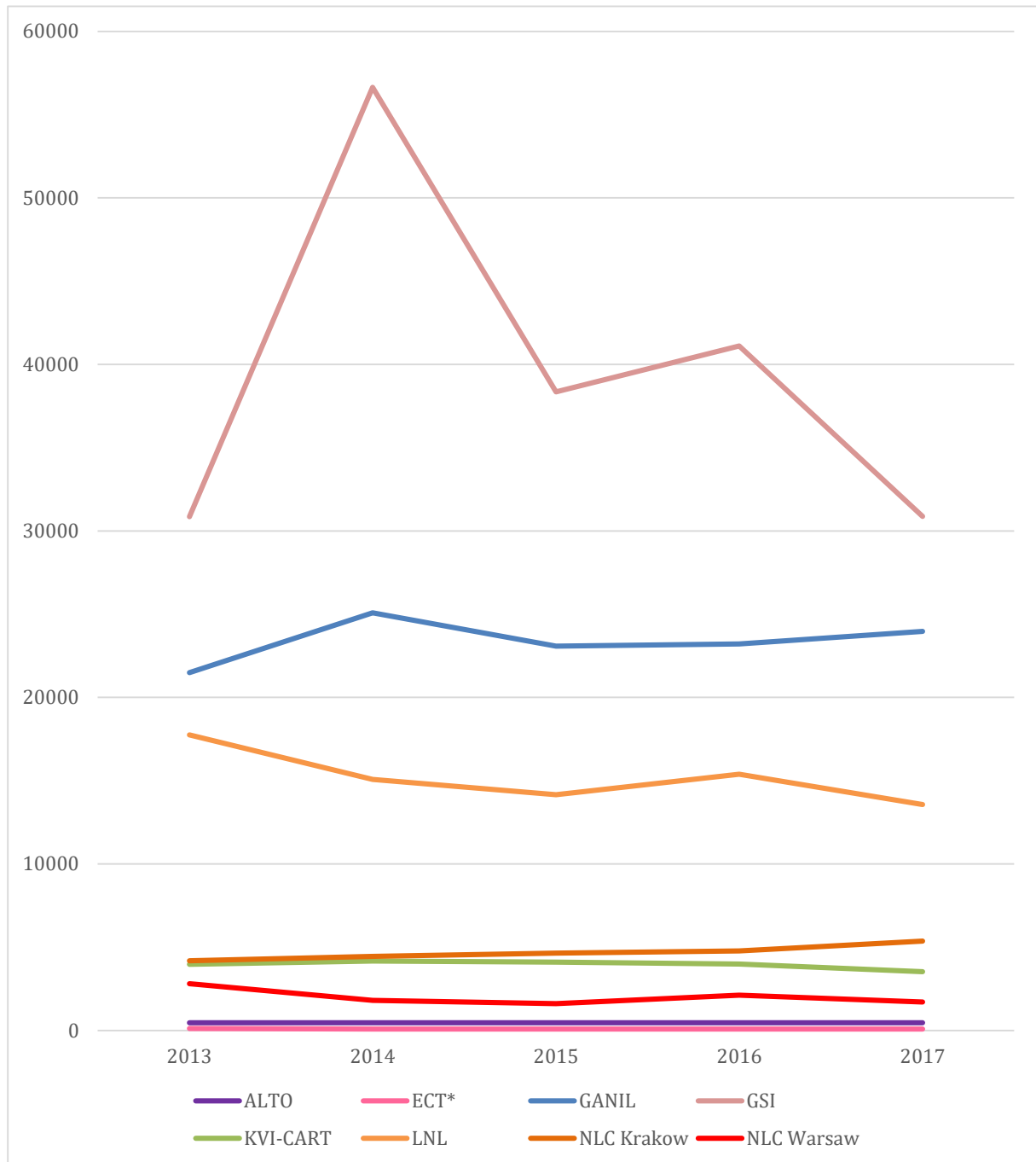
Figure 17 : Electricity consumption in MWh 2013-2017 (data from ALTO, ECT*, GANIL, GSI, KVI-CART, LNL, NLC Krakow and NLC Warsaw)
